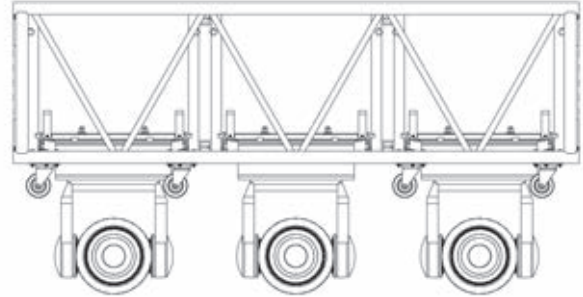
Front View with Lights in lowered position
